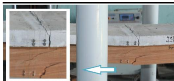
Fig. 10 specimen TF6 after failure
