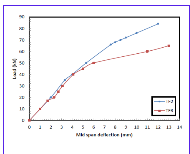
Fig. 16 Variation of midspan deflection with load for composite beams sag moment and hog moment with dimension of timber (135x85)
