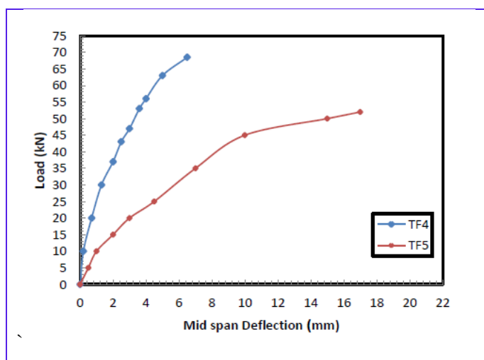
Fig. 15 Variation of midspan deflection with load for composite beams sag moment and hog moment with dimension of timber (85x85)
