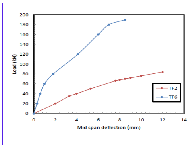
Fig. 13 Variation of midspan deflection with load for composite beams The variable is timber depth
