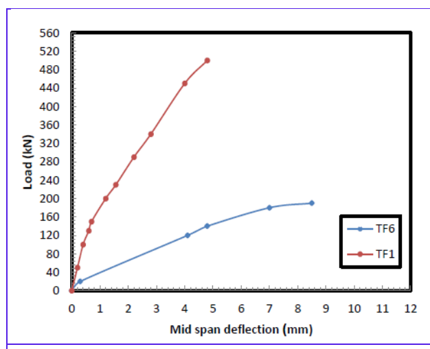
Fig. 14 Variation of midspan deflection with load for composite beams The variable is timber width
