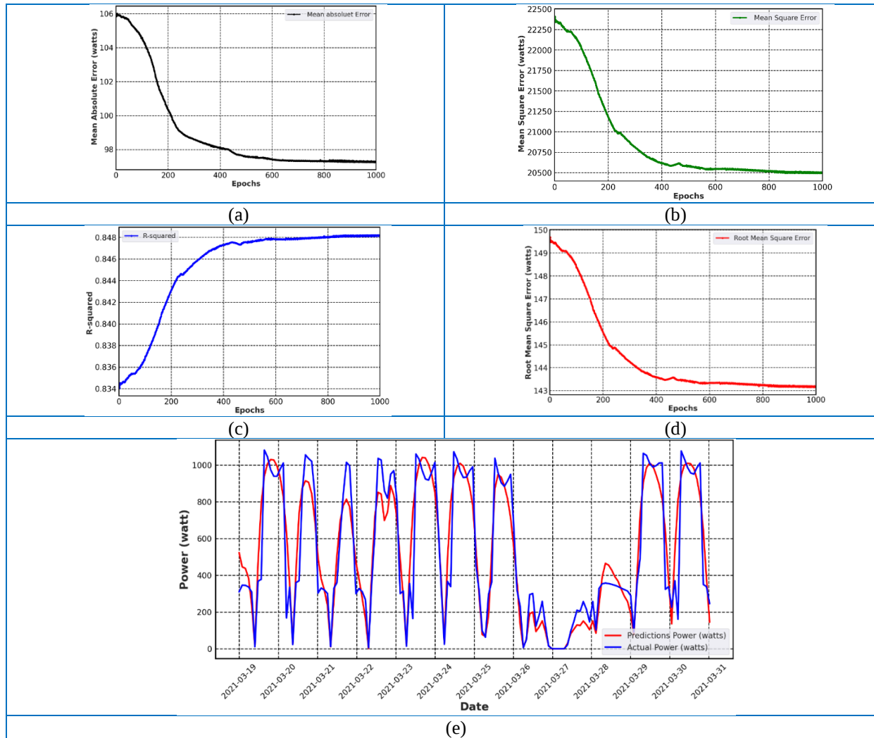
Fig. 8. The results of March of (a) MAE, (b) MSE, (c)R2, (d) RMSE, and (e) the relationship between actual power and prediction power
